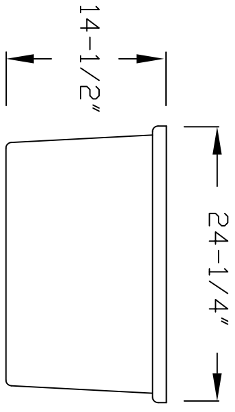
BOX SECTION VIEW
